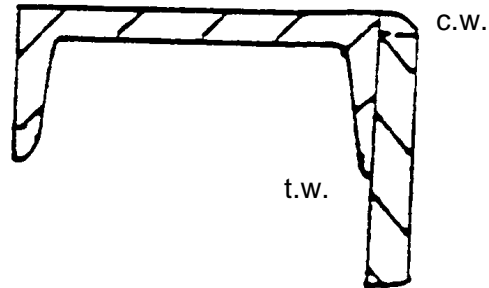
Curb Construction
