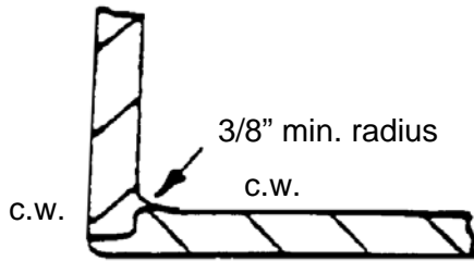
Preferred Corner Construction
