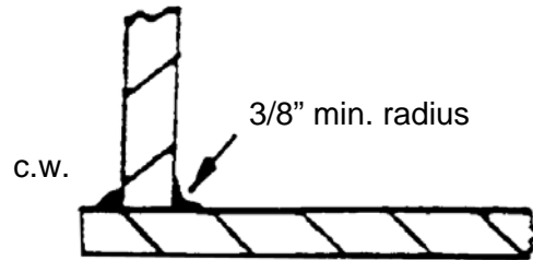
Acceptable Corner Construction
